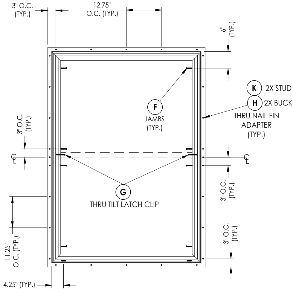
FRAME ANCHORING
