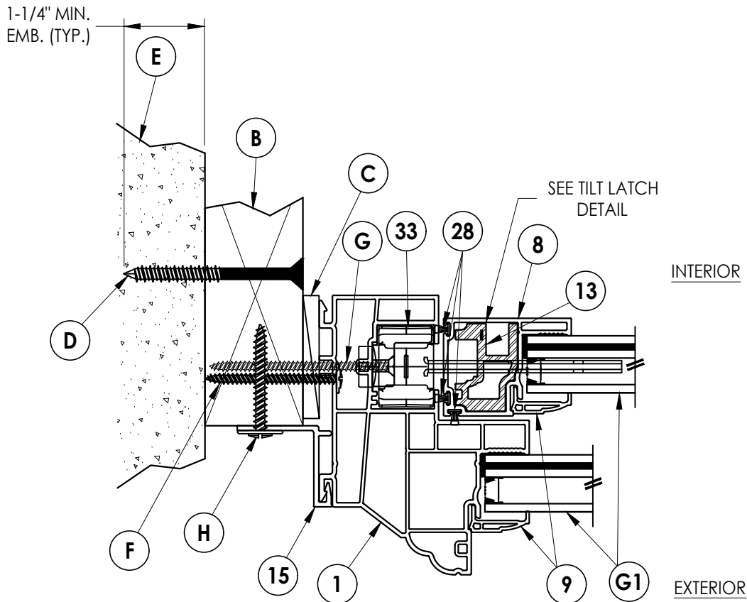
1 HORIZONTAL CROSS SECTION 2 2X Buck Construction
